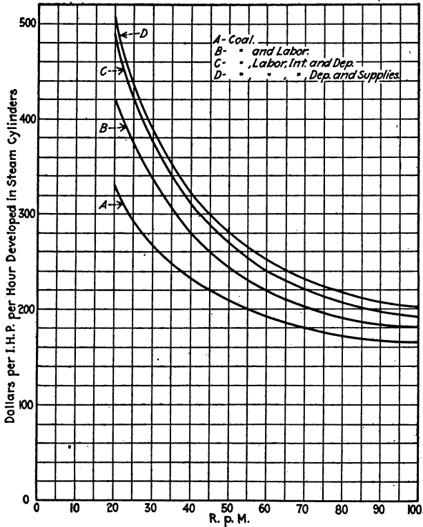
FIG. 121.—Test results of compressor plant No. 2.
